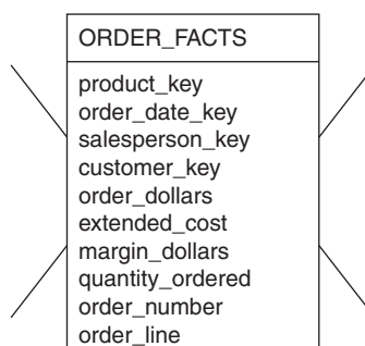
Figure 10-11 Inside a fact table.
