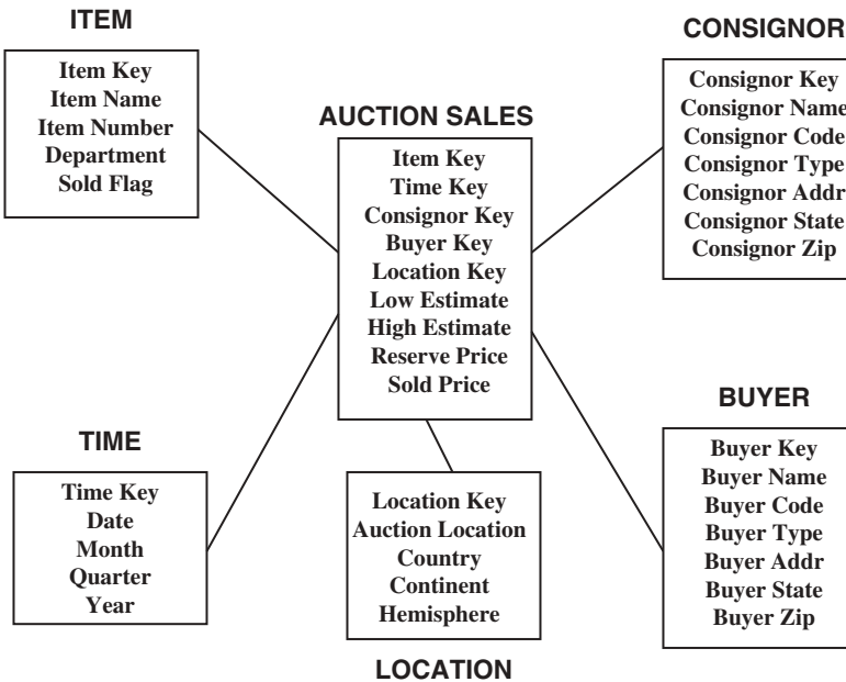
Figure 10-18 STAR schema example: auction company.
