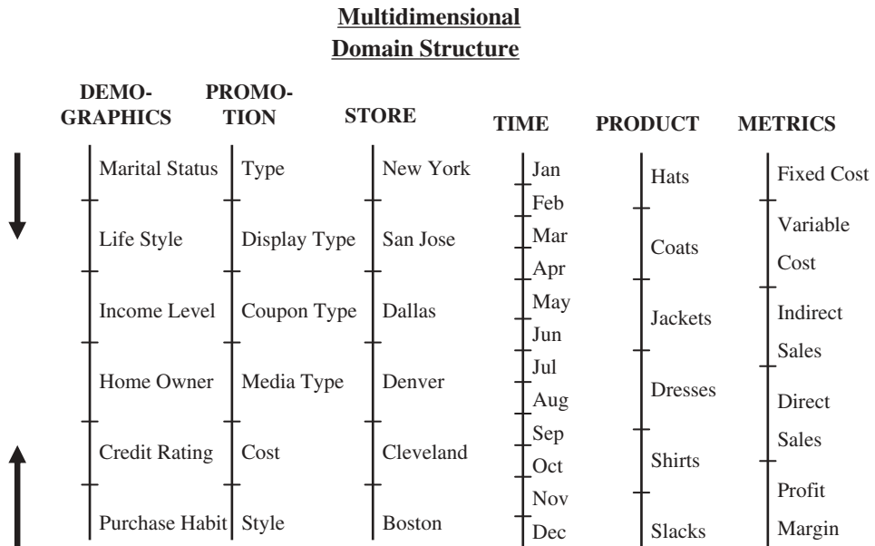
Figure 15-10 Six-dimensional MDS.
