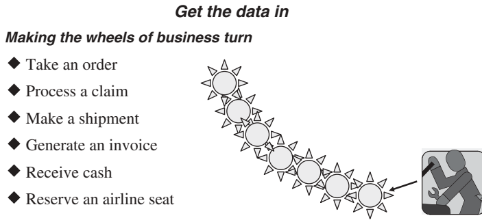
Figure 1-5 Operational systems.
