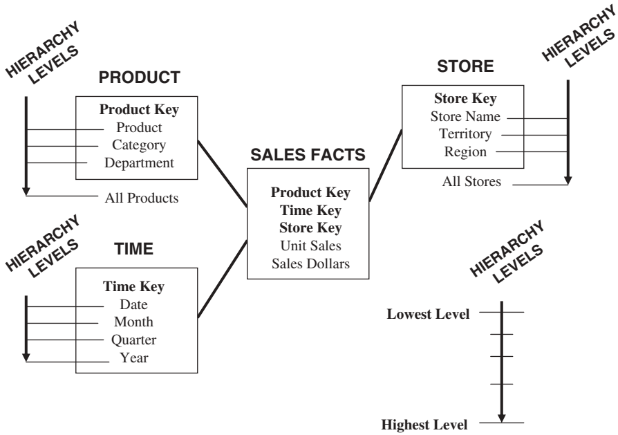
Figure 11-13 Dimension hierarchies.
