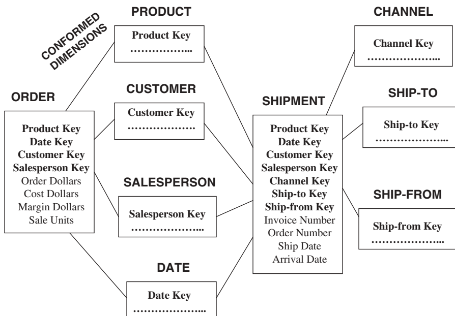
Figure 11-19 Conformed dimensions.
