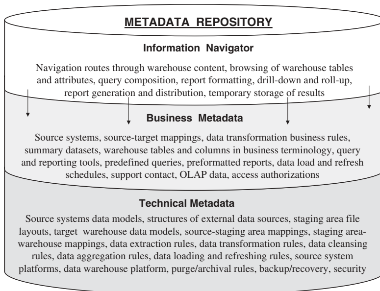
Figure 9-11 Metadata repository.
