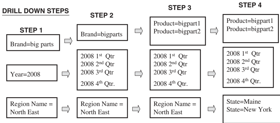
Figure 10-9 Understanding drill-down analysis from the STAR schema.
