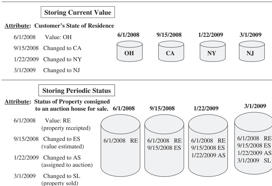
Figure 12-3 Data in operational systems.
