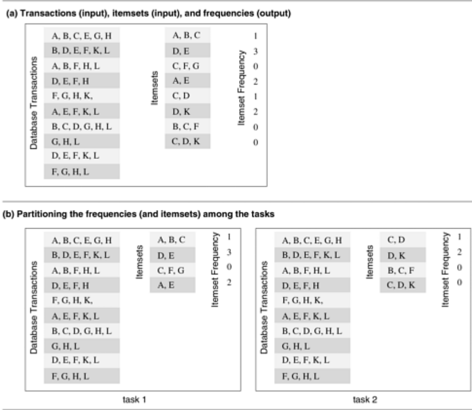
Figure 3.12(b) shows how the computation of frequencies of the itemsets can be decomposed into two tasks by partitioning the output into two parts and having each task compute its half of the frequencies. Note that, in the process, the itemsets input has also been partitioned, but the primary motivation for the decomposition of Figure 3.12(b) is to have each task independently compute the subset of frequencies assigned to it.
